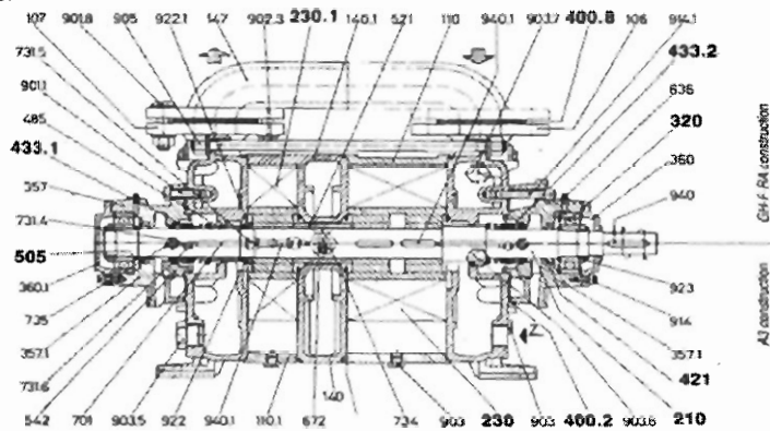
Typical Cross Section with Mechanical Seal
